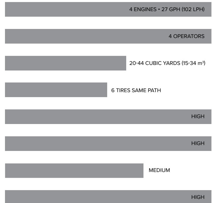
EXCAVATOR + ARTICULATED DUMP TRUCKS + DOZER
